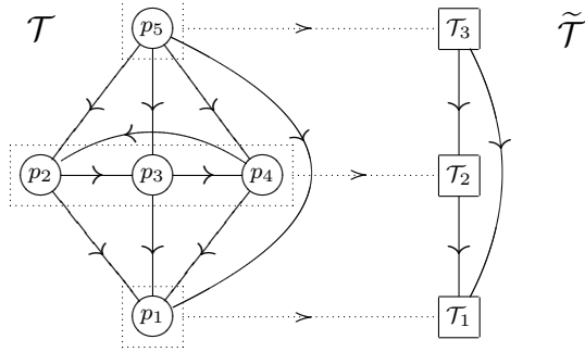
Figure 1: The condensation of a tournament.
