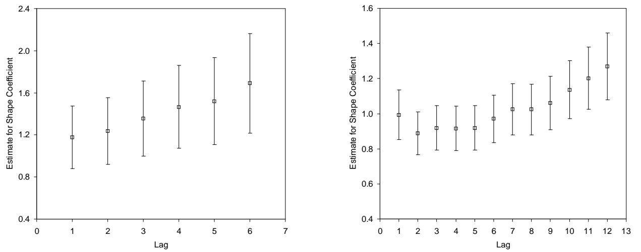
Figure 7: Increasing the time lag in the computation of growth rates. Estimates of the shape coefficient ( \hat{b} ). Left: US GDP. Right: US IP1947. Bars represent Cramer-Rao intervals ( \hat{b} \pm 2\sigma(\hat{b}) ).
