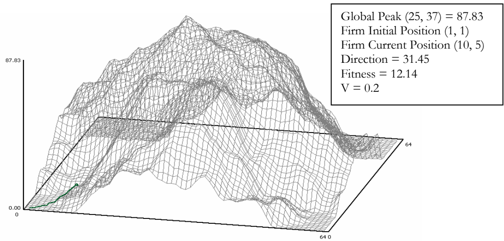
Figure 1: Searching a Rugged Landscape, Differing Values of v h = 1.25 , No Tilt, Number of Periods = 500
