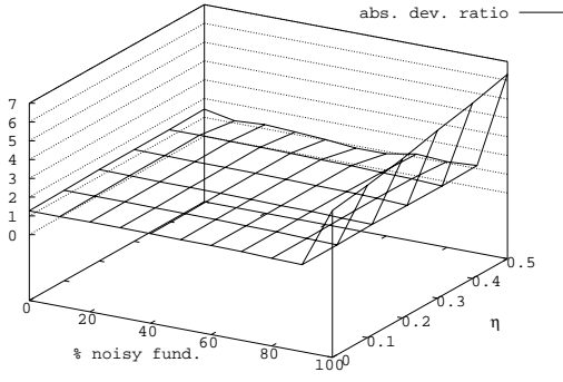
Figure 9: Ratio of returns absolute deviations in the batch and order book protocols. The statistics are computed for different proportion of agents types and for different values of \eta .
