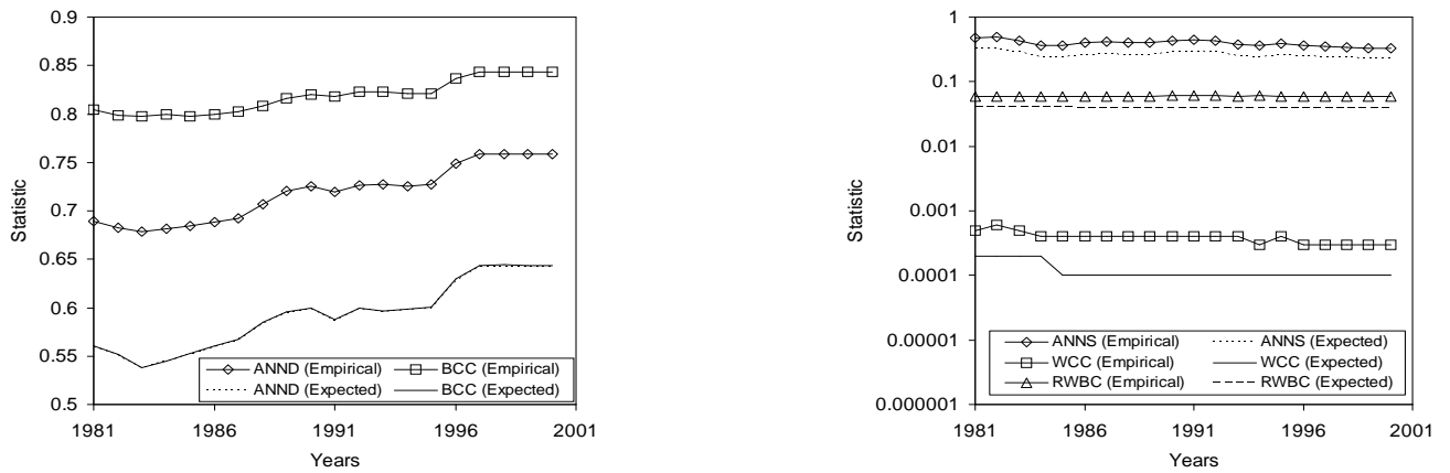
FIG. 9: Population average vs. expected values of node statistics. Expected values for binary-network statistics (left) are computed by reshuffling binary links by keeping observed density fixed. Expected values for weighted-network statistics (right) are computed by reshuffling observed link weights while keeping the binary structure fixed.
