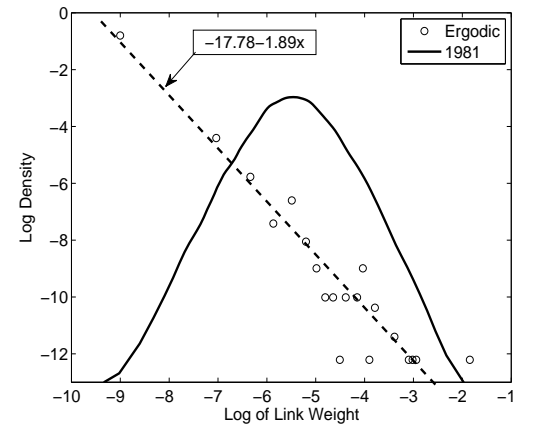
FIG. 17: Positive link weights: Kernel density of initial distribution (year=1981) vs. estimate of ergodic (limiting) distribution. Dotted line: Power-law fit (equation shown in inset). Note: Log scale on y-axis.
