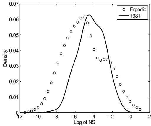
FIG. 16: Node Strength (NS): Kernel density of initial distribution (year=1981) vs. estimate of ergodic (limiting) distribution.
