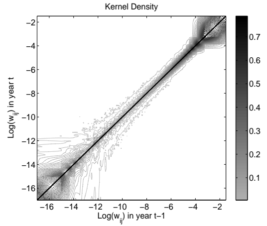
FIG. 13: Contour plot of stochastic-kernel estimates for logged positive link-weights ( \log(w_{ij}^t), w_{ij}^t > 0 ). Solid line: Main 45° diagonal.
