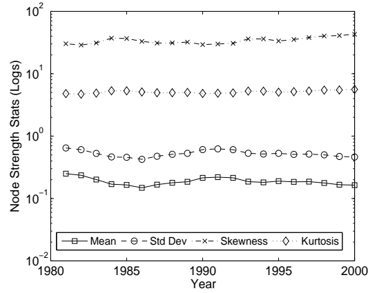
FIG. 3: Sample moments of the node strength (NS) distribution vs. years. Log scale on Y-axis.
