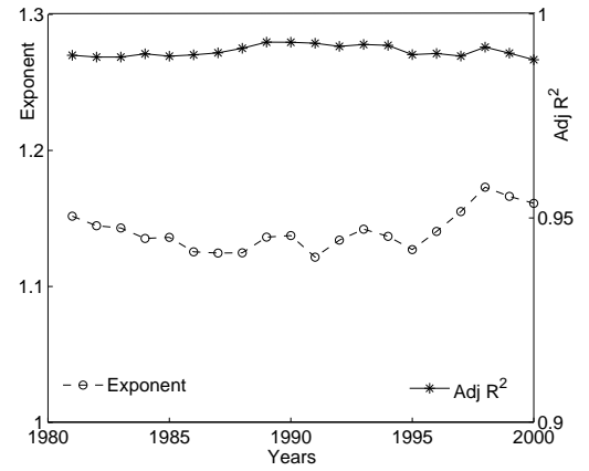
FIG. 7: Left Y-axis scale: Estimated power-law exponent for node random-walk betweenness centrality (RWBC) distributions vs. years. Right Y-axis scale: Adjusted R^2 associated to the power-law fit.
