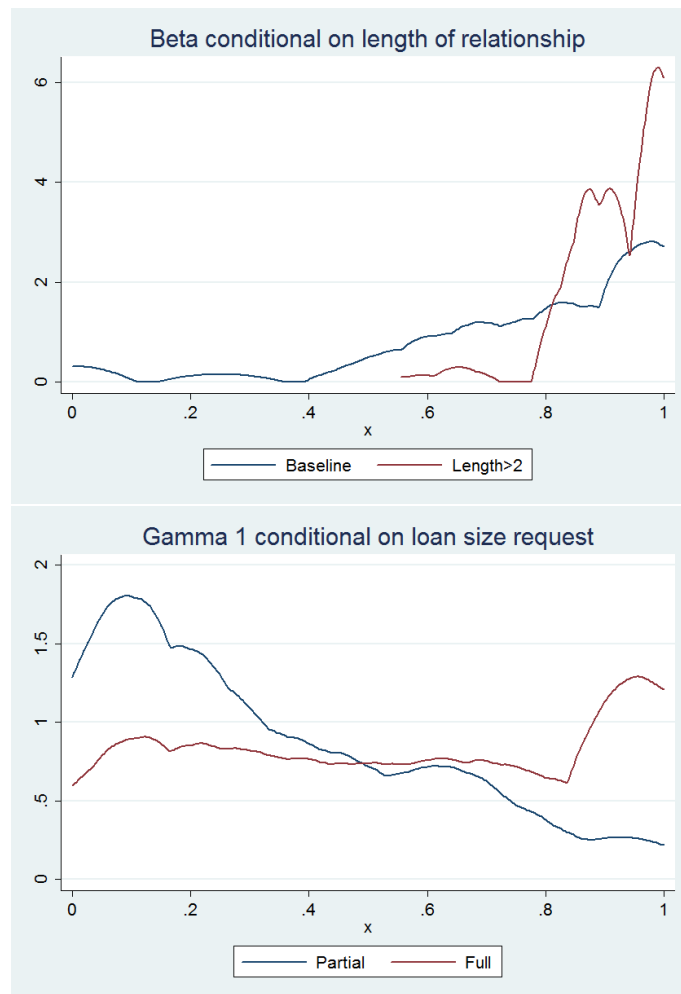
Figure 9: Conditional distributions
