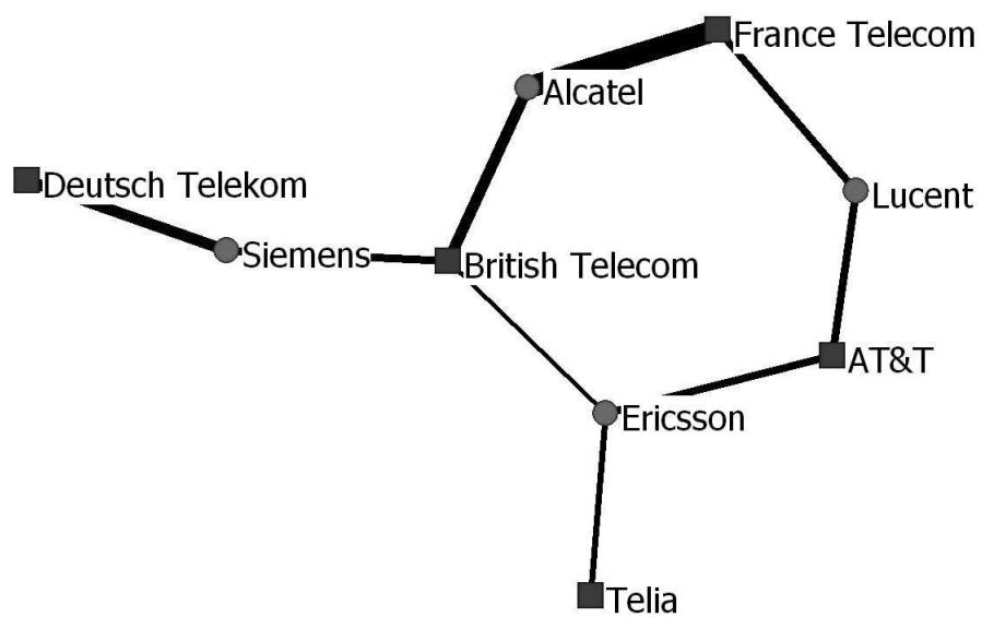
Figure 1: A two-mode network. An example.
