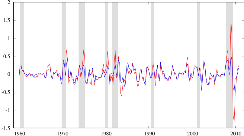
Figure 1: The Threshold Variable: the MA(2) of the first difference of the spread between BAA-rated corporate bond yields and 10-year treasury constant maturity rate (red line) and the MA(2) of the first difference of the spread between AAA-rated corporate bond yields and 10-year treasury constant maturity rate (blue line). Shaded areas: recession periods according to the NBER business-cycle chronology.
