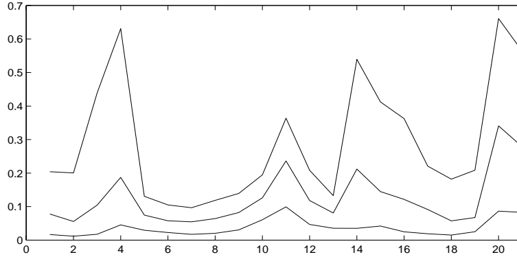
Figure 4.1 Variance-ratio of idiosyncratic component to the variable
