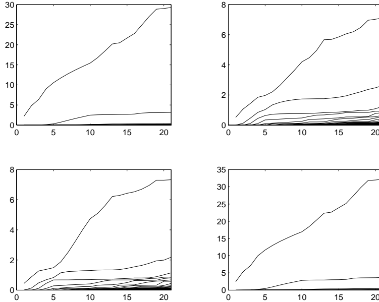
The graphs in the first row, from the left, correspond to the frequencies 0, \pi/3 , in the second row to 2\pi/3, \pi .
