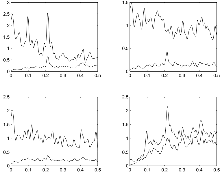
The variables in the first row, from the left, are nfcpl and ed1, respectively. The second row reports t10 and ffr, respectively. Cycles per day on the horizontal axis.
