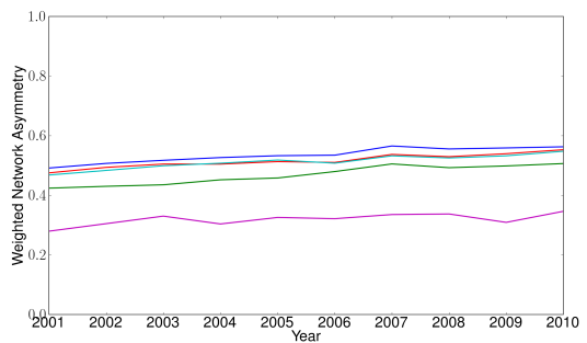
(f) Relative weighted network asymmetry
