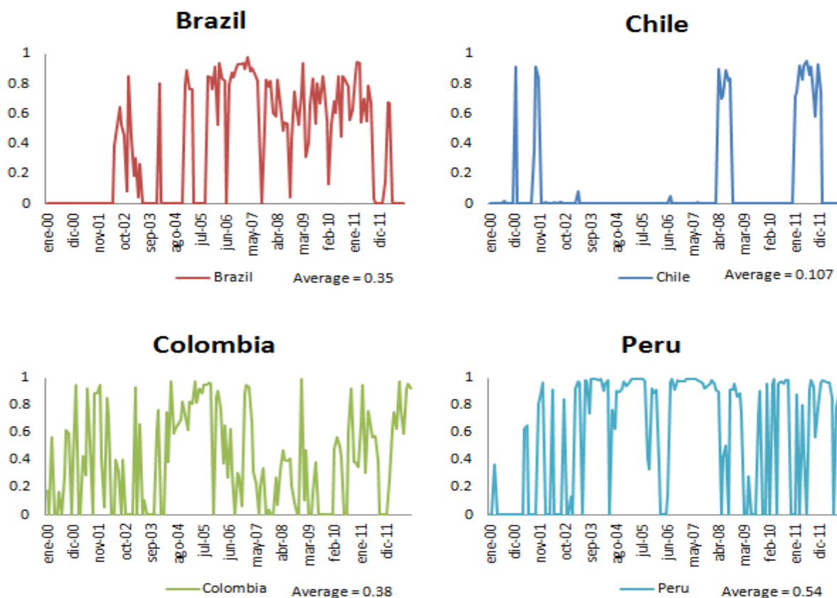
Figure 4. Intervention Index
