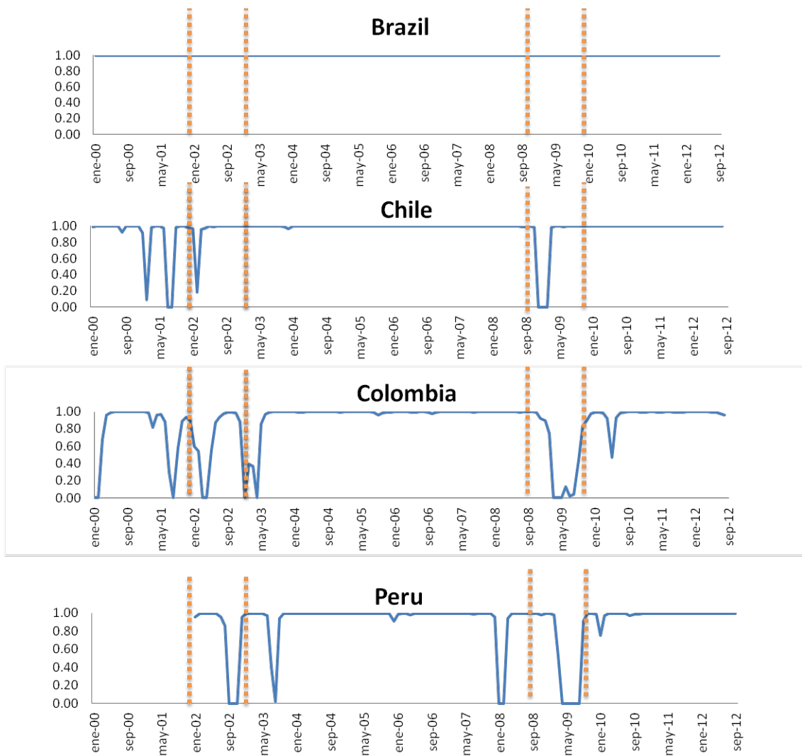
Figure 2. Regime Switching
