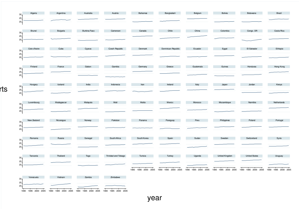
Figure 2: Time series plots for \ln(\text{imports})
