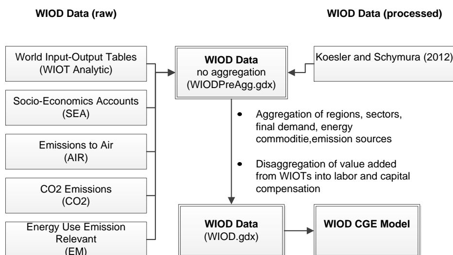
Figure 1: Data Structure
