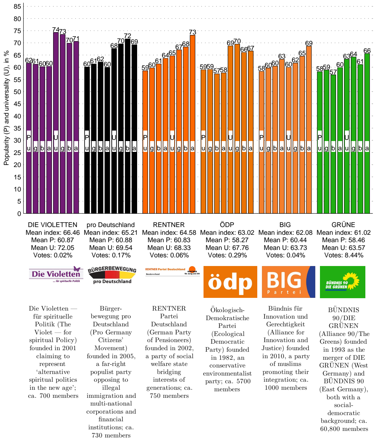
Figure 2: Sheet C. Indices of German parties and the DGB: P—popularity, U—universality, u—for unweighted questions, g—for questions weighted by the number of Google hits, b—for questions weighted by Brigitte Unger as the first expert, and a—for questions weighted by Anne Graef as the second expert
