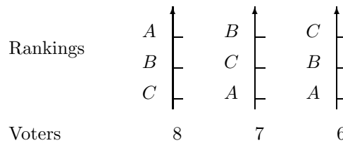
Figure 1: Borda’s example from 1770 as given by [Black 1958, p. 157]
