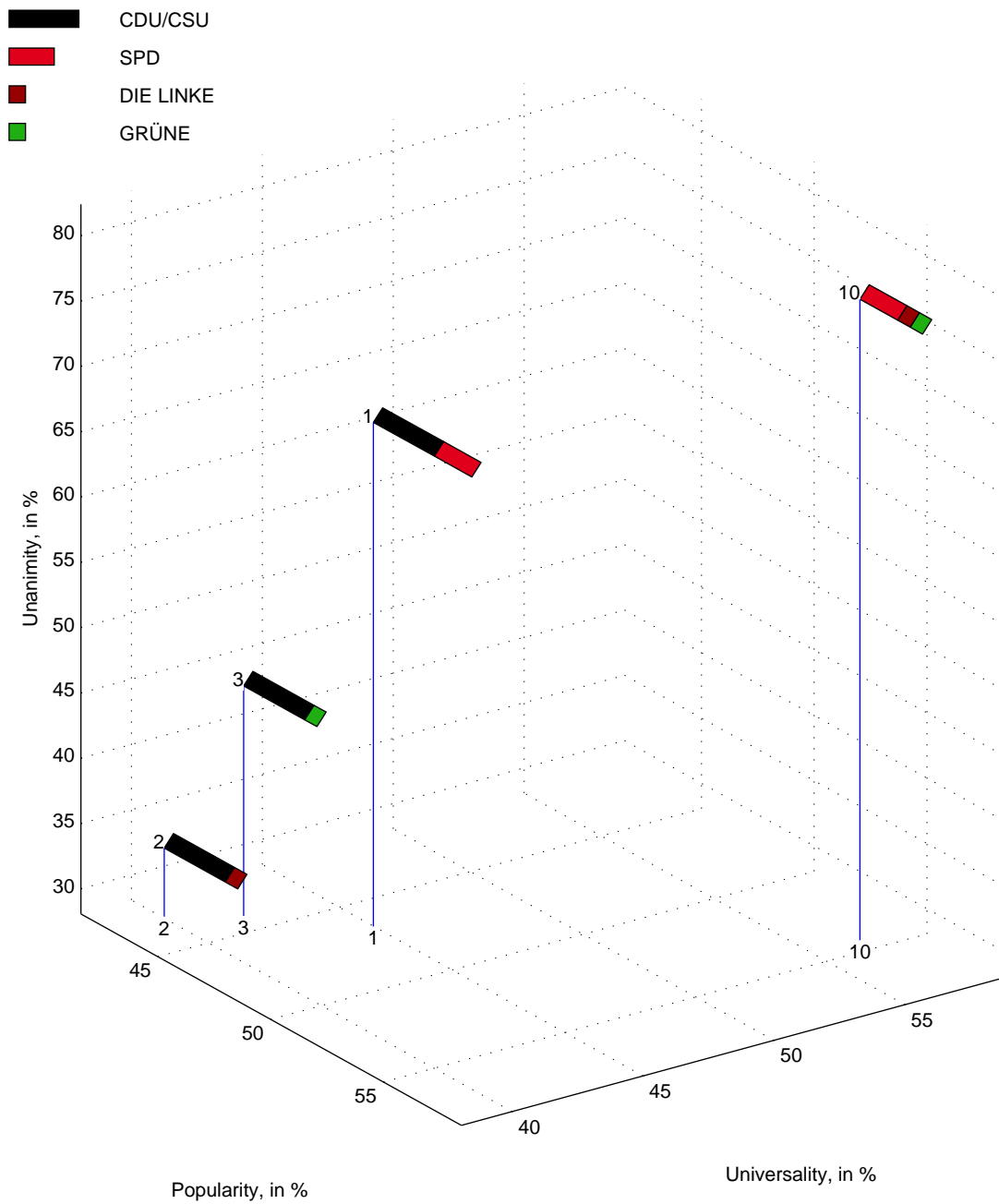
Figure 5: Indices of minimal eligible coalitions (with > 50\% parliament seats); the indices are computed for unweighted questions, and the impact of member weights on the coalition decisions is assumed to be p = 0.50
