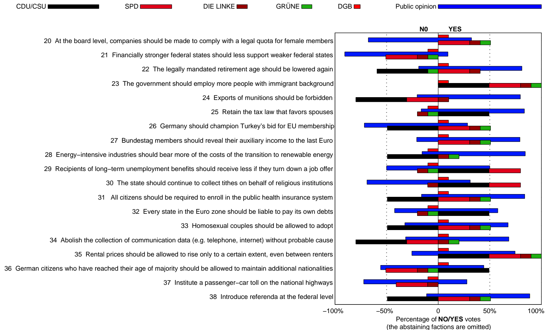
Figure 3: Sheet B. Public opinion and representation thereof by the 2013 Bundestag and the DGB
