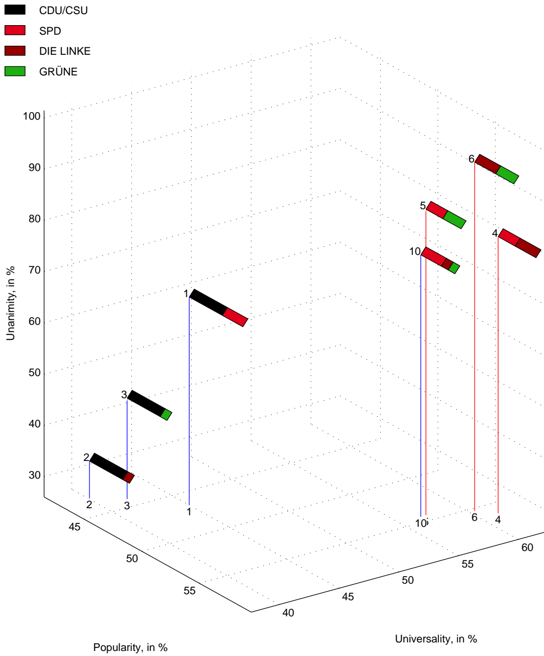
Figure 7: Actual minimal eligible coalitions — with > 50\% parliament seats (shown by blue flagstuffs) and recalculated minimal eligible coalitions (shown by red flagstuffs); in both cases the indices are computed for unweighted questions, and the coefficient of impact of member weights on the coalition decisions is assumed to be p = 0.50
