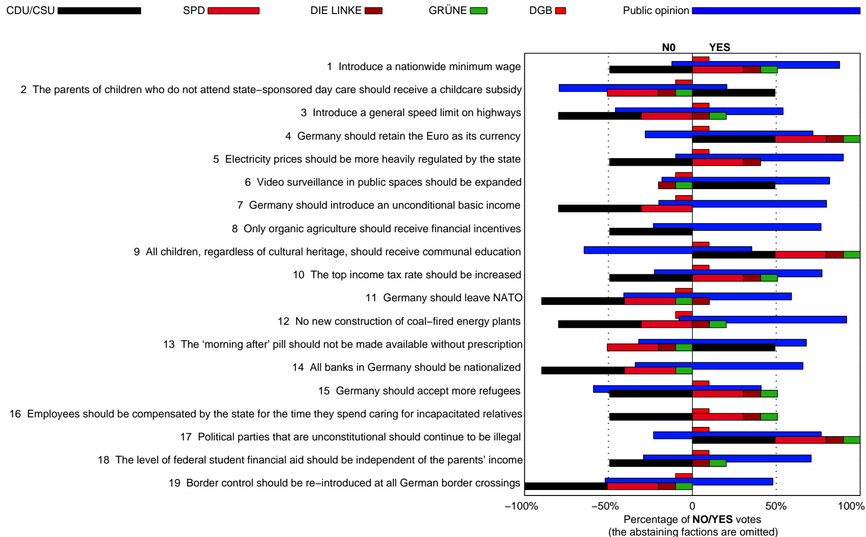
Figure 3: Sheet A. Public opinion and representation thereof by the 2013 Bundestag and the DGB
