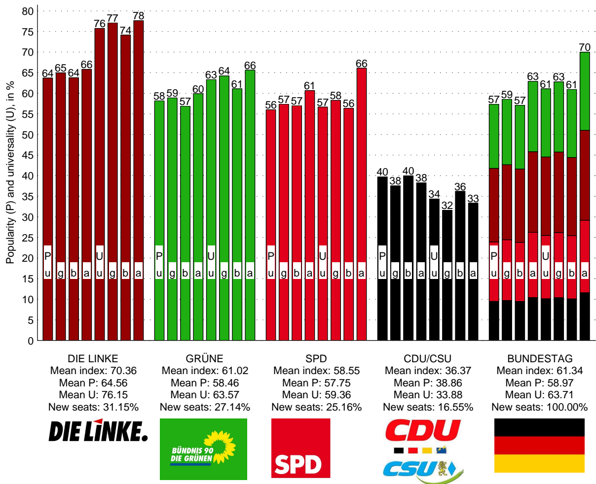
Figure 6: Indices of the four eligible parties and of the Bundestag with the seats redistributed proportionally to the mean indices of the parties: P—popularity, U—universality, u—for unweighted questions, g—for questions weighted by the number of Google hits, b—for questions weighted by Brigitte Unger as the first expert, and a—for questions weighted by Anne Graef as the second expert
