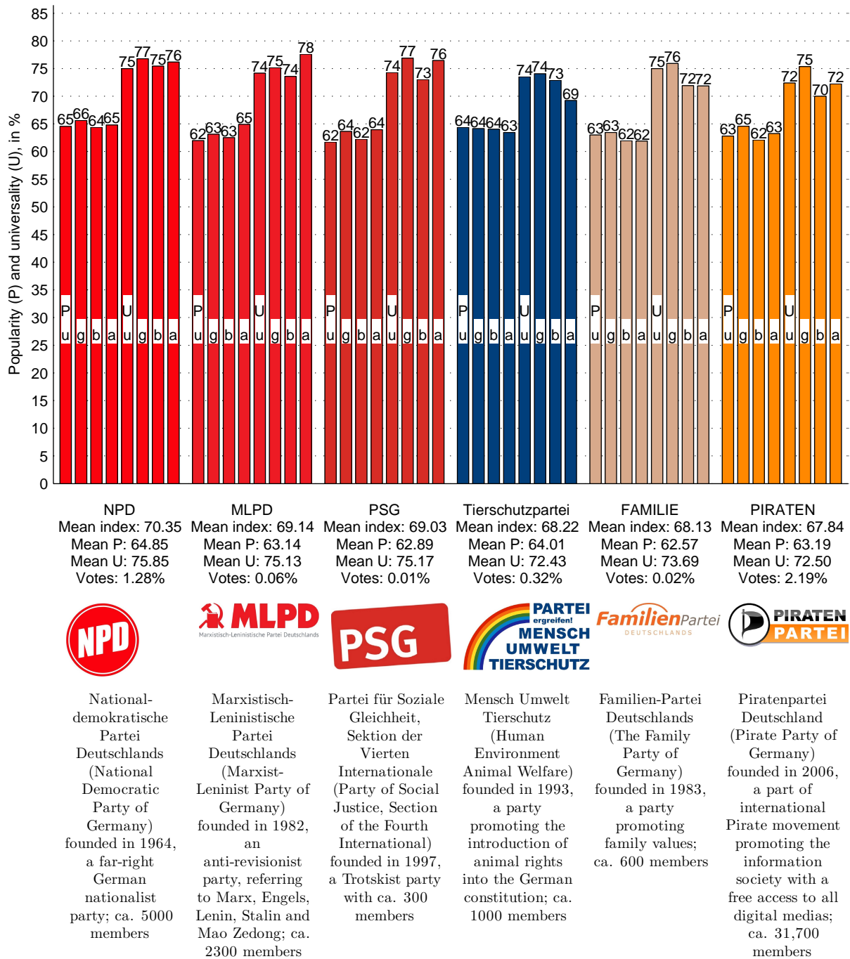
Figure 2: Sheet B. Indices of German parties and the DGB: P—popularity, U—universality, u—for unweighted questions, g—for questions weighted by the number of Google hits, b—for questions weighted by Brigitte Unger as the first expert, and a—for questions weighted by Anne Graef as the second expert
