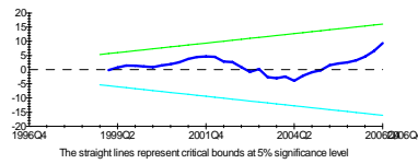
Plot of Cumulative Sum of Recursive Residuals
