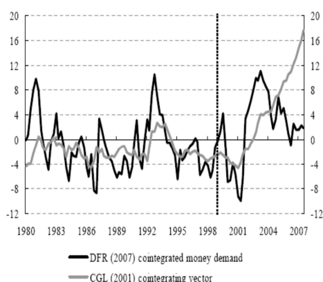
Figure 3: Residual of a standard money demand specification based on Calza et al. (2001)
