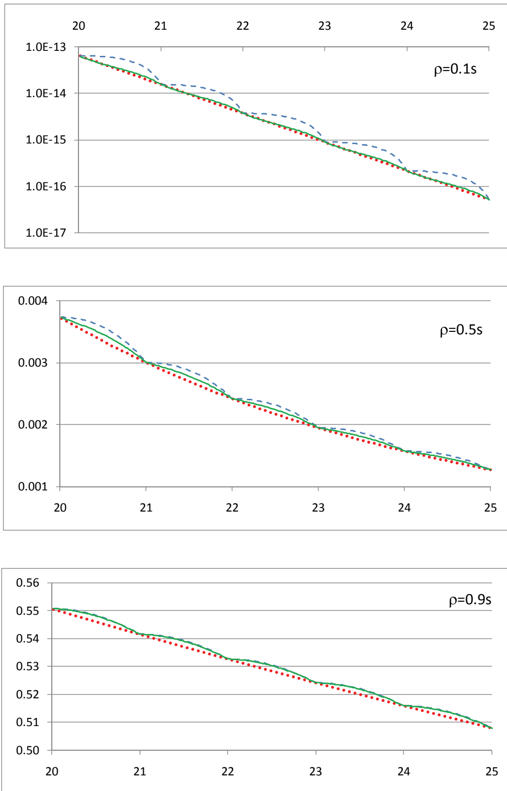
Figure 3. Probability of delay C_{R(s),s}(\rho) for 20 \leq s \leq 25 ,
