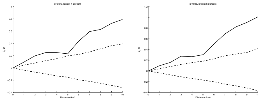
Figure 7: D -function
