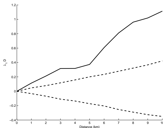
Figure 4: D -function
