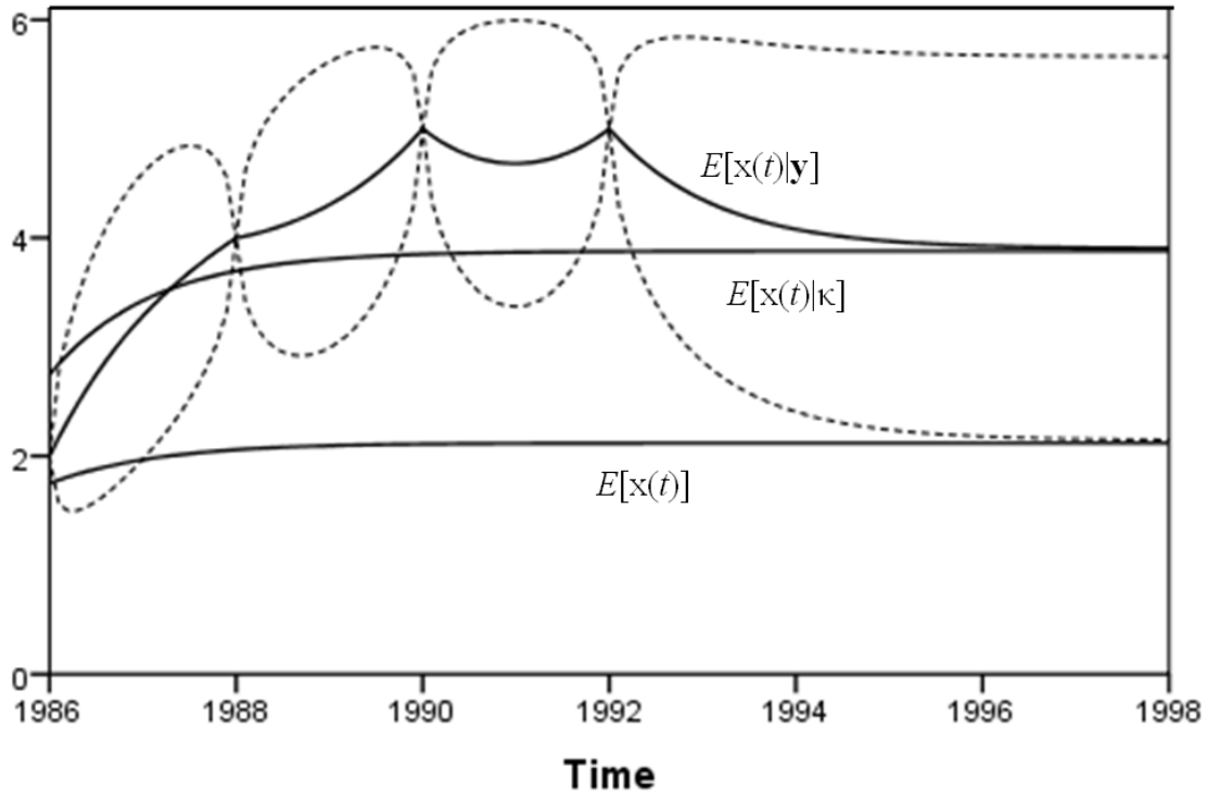
Figure 1. Estimated mean curve E[\mathbf{x}(t)] , subject-specific mean curve E[\mathbf{x}(t)|\kappa] and sample trajectory curve E[\mathbf{x}(t)|\mathbf{y}] (for the same subject as in E[\mathbf{x}(t)|\kappa] ) in CT (confidence intervals for the sample trajectory curve represented by dotted lines)
