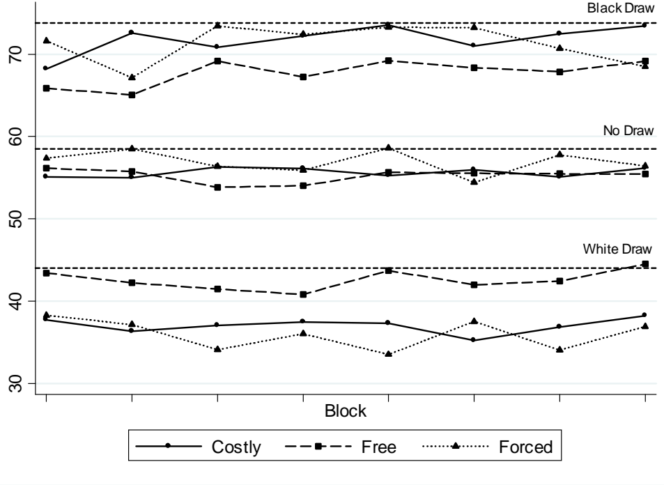
Figure 4: Average decisions by periods. Note: Decision averages for each block are calculated using all decisions made in a 5 period interval (8 blocks of 5 periods) by all subjects within an information type. For example, the top solid line oscillating around 70 represents the 5 period average of subjects' decisions who drew a Black ball in the Costly treatment. The dashed straight lines denote the Bayesian benchmark.
