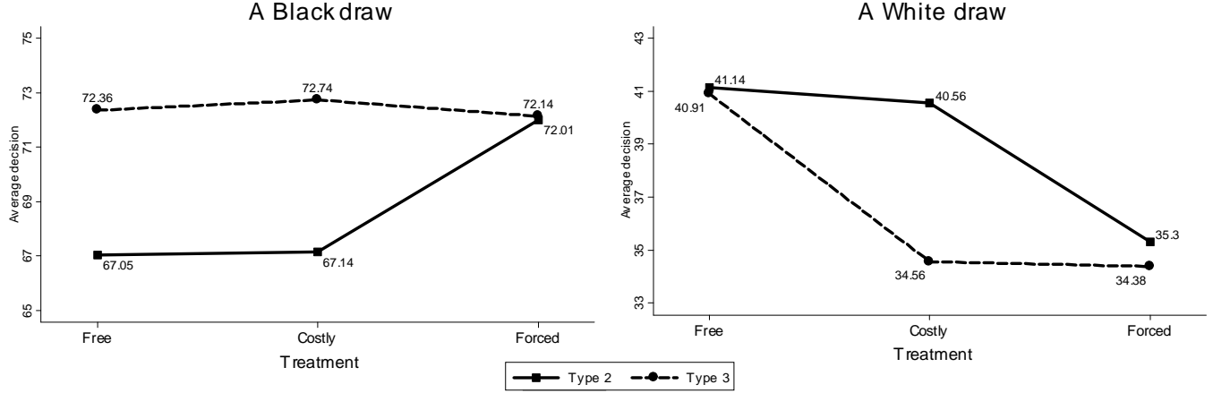
Figure 6: Average decision by subject type.
