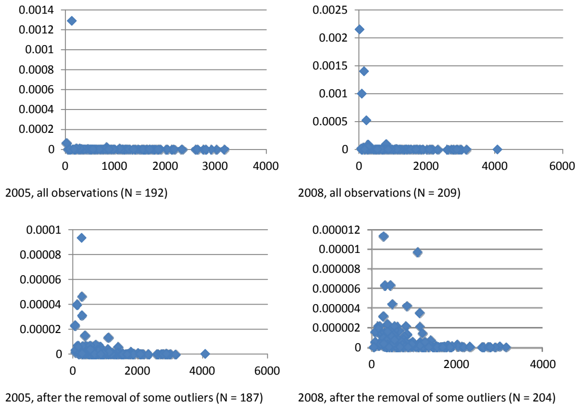
Figure A1: Plots of the impedance functions, 2005 and 2008: y-axis = , x axis =
