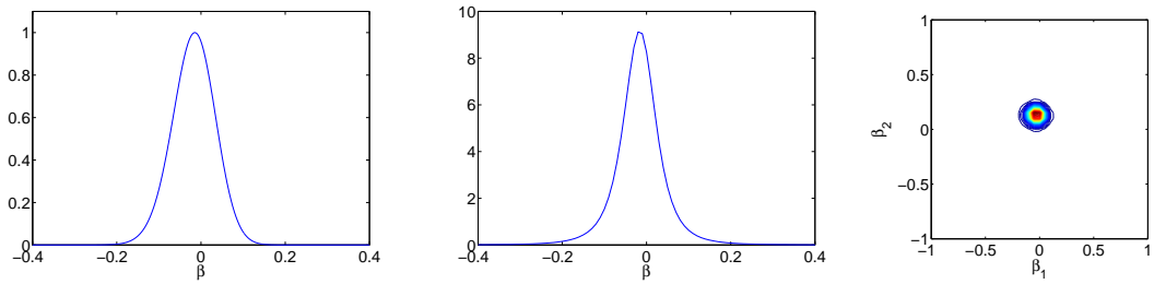
Figure 6. Marginal posterior of \beta in case 3 ( k = 4 strong instruments for m = 1 moderately endogenous regressor): posterior density kernel (left); candidate density (mixture of 2 Student- t densities) (middle).
