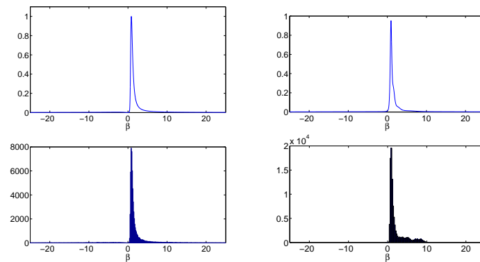
Figure 8. Marginal posterior of \beta for example due to Acemoglu et al. (2001): posterior density kernel (top left); candidate density (mixture of 8 Student-t densities) (top right); histogram of ARDMC draws (bottom left); histogram of Gibbs draws (bottom right).
