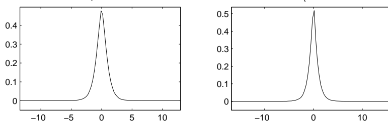
FIGURE 2. Densities for the simulated distributions (no volatility feedback).
