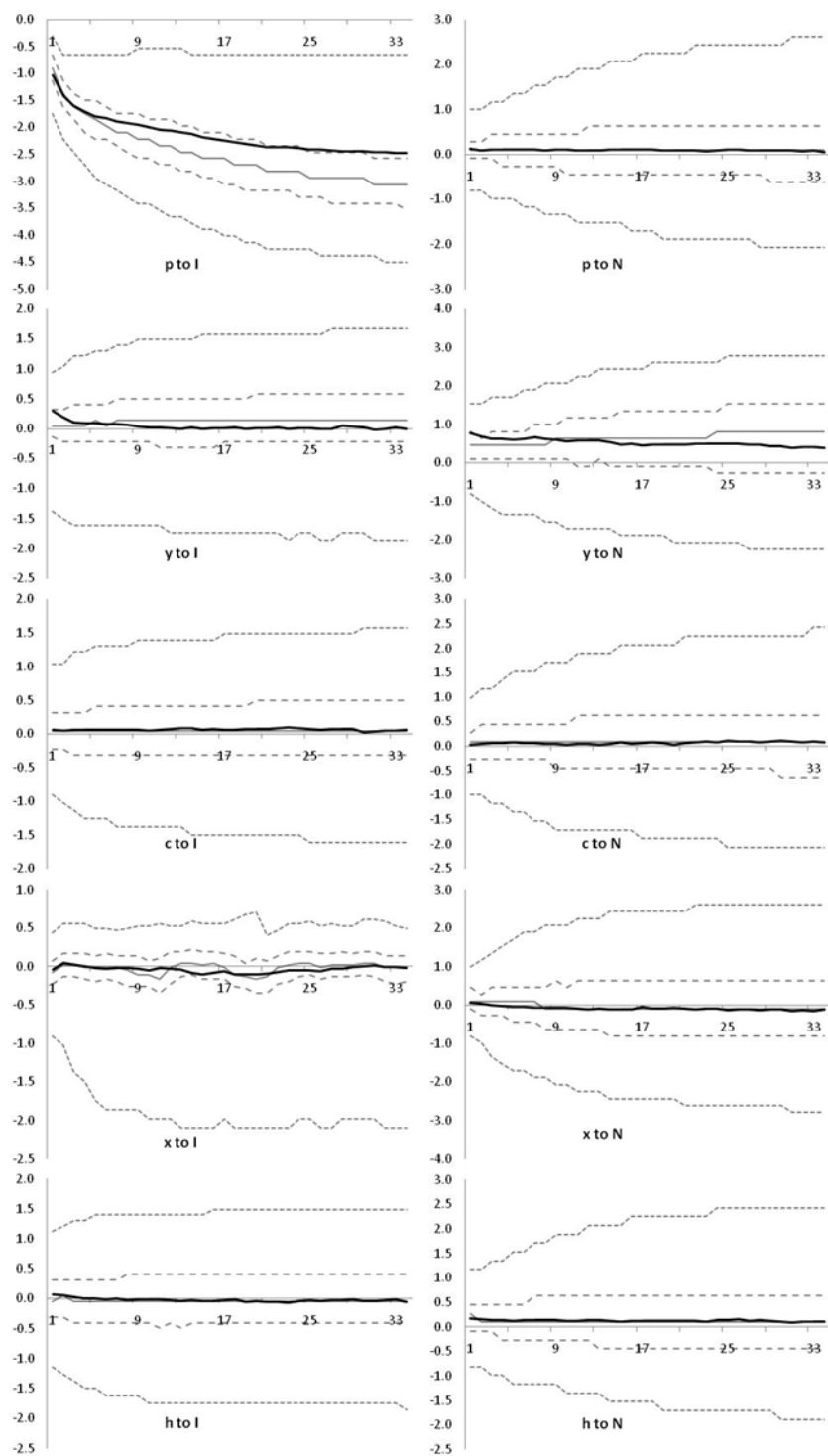
Figure 3: The 20%, 40%, 50%, 60% and 80% percentiles of the posterior distribution of the response of investment price, p , output, y , consumption, c , investment, x , and hours, h , to investment specific, I , and neutral, N , technology shocks. The x-axis is periods since the shock and the y-axis is in percent.
