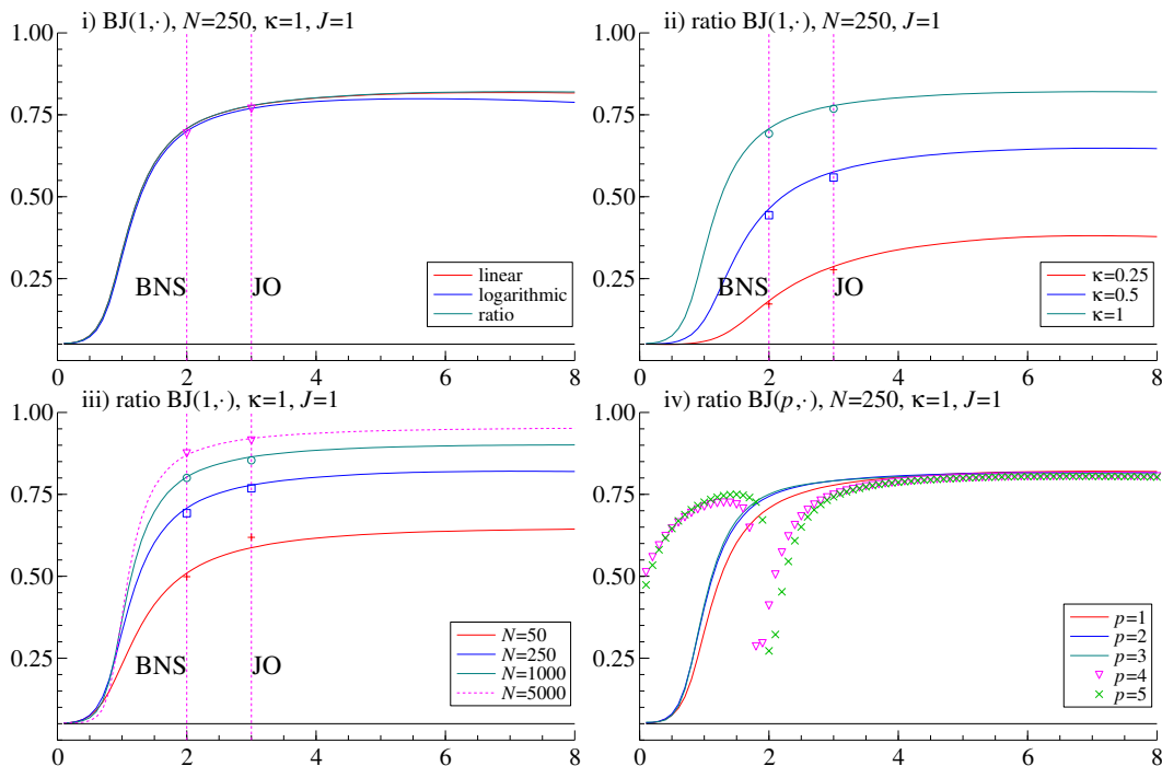
Figure 5: Distribution under the alternative
