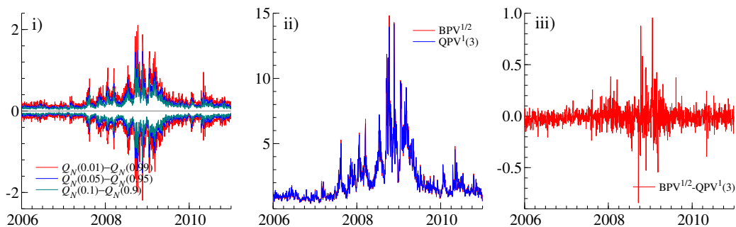
Figure 6: Empirical quantiles and variation measures
