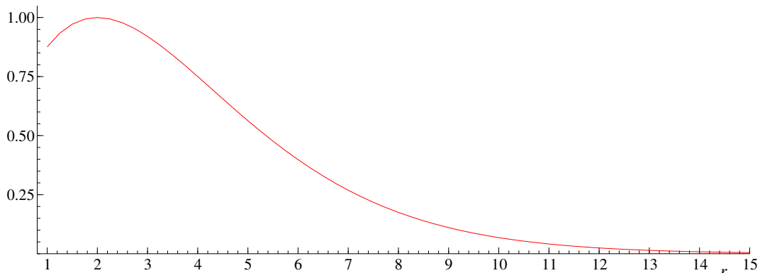
Figure 1: Efficiency of MPV relative to ML
