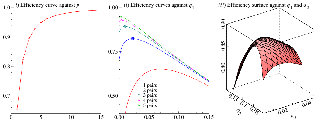
Figure 2: Efficiency of QPV_N(\mathbf{q}, \boldsymbol{\lambda}) relative to the maximum likelihood estimator
