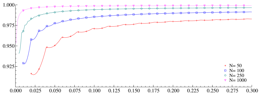
Figure 3: Finite sample correction \Phi^{-1}(q)/\bar{Q}_N^N(q)
