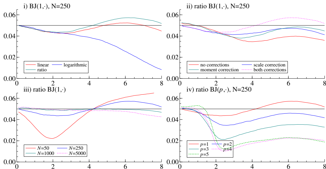
Figure 4: Size characteristics of BJ tests
