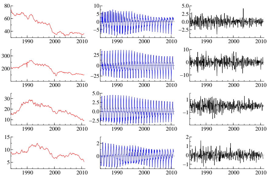
Figure 7: Trend (left), seasonal (middle), and irregular (right) components in property crime rates: burglary (first row); larceny (second row); motor vehicle theft (third row); robbery (fourth row).
