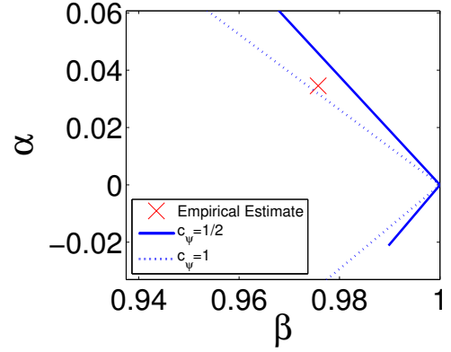
(b) Gaussian estimates ( a = 1 )
