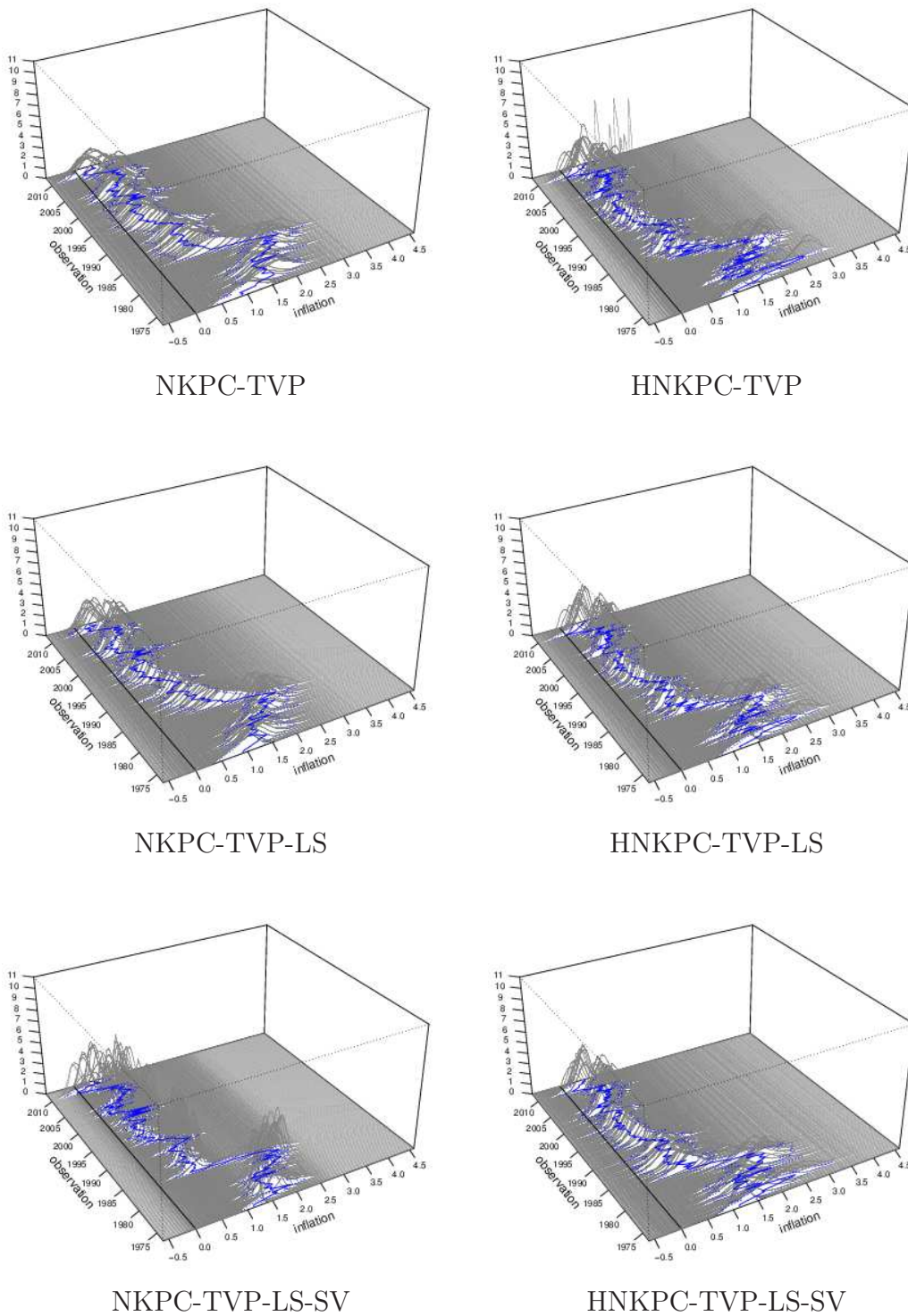
Figure 11: Predicted inflation densities from NKPC and HNKPC models
