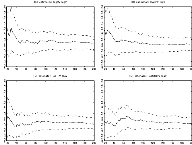
Figure 3: Hill estimator of the right tail dependence, X -axis measures n_u = 20, \dots, 200 .
