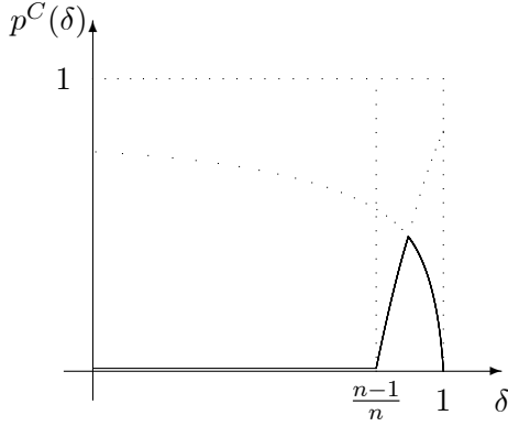
Figure 1: The profit-maximizing cartel price p^C(\delta) .
