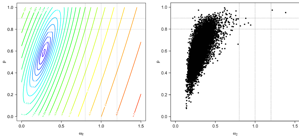
Figure 8: Left: contour plot of the (natural) logarithm of the t_1 candidate density. Right: 50'000 draws from the marginal distribution of (\omega_2 p)' obtained with the t_1 M-H strategy (i.e., using a t_1 approximation as the candidate density in the independence chain M-H algorithm).
