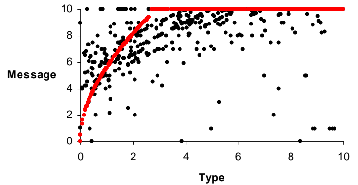
Message on type, last 20 periods, b=4
