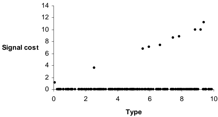
Signal cost on type, period 36-45, hybrid b=1
