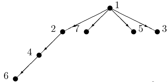
Figure 3: Hierarchy (N^6, S^6)
