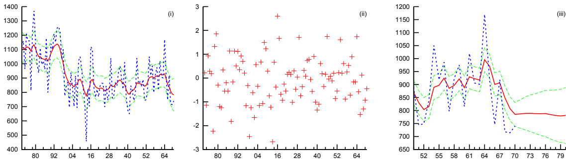
Figure 2: Nile data, with smoothed state and 90% confidence interval (panel (i)), standardised prediction errors (panel (ii)), and filtered state plus forecast with 50% confidence interval (panel (iii))
