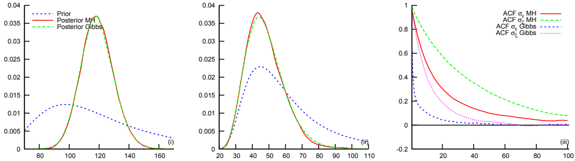
Figure 1: Prior and posterior densities for \sigma_\varepsilon (panel (i)) and \sigma_\xi (panel (ii)) for the Nile data, with autocorrelations in panel (iii), comparing MH and Gibbs results
