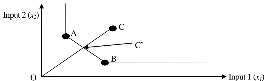
Figure 1. Illustration of original DEA projection in Input space
