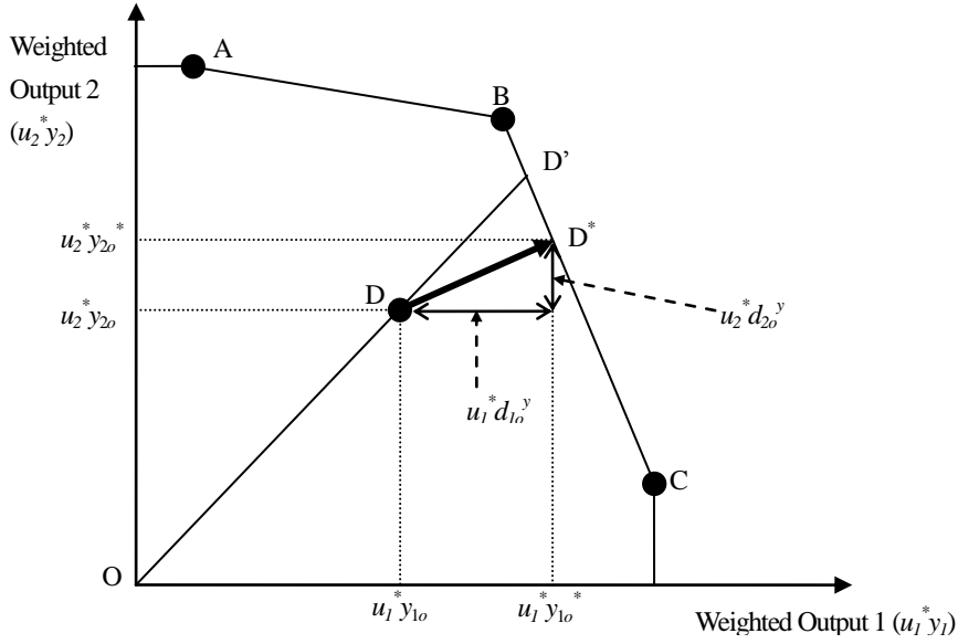
Figure 3. Illustration of DFM approach (Output- u_r y_r space)
