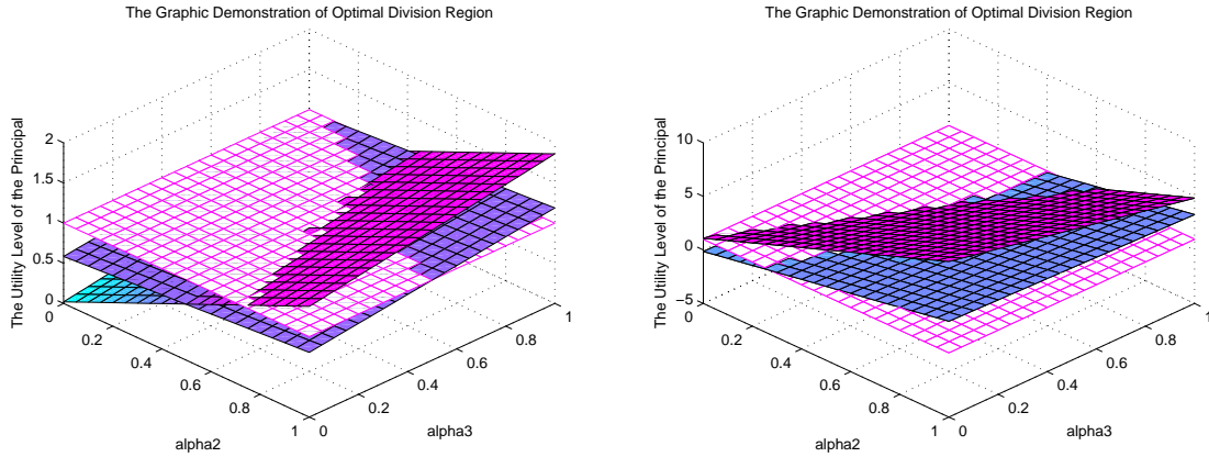
Figure 6: The principal's benefit when \gamma_1 = 0.1, \gamma_2 = w = 0.5 (left) and \gamma_1 = 0.9, \gamma_2 = w = 0.5 (right). The pink surface with black grid is the utility under agent 2 control, the white surface with pink grid is under agent 1 control and the purple one is her utility under separation.
