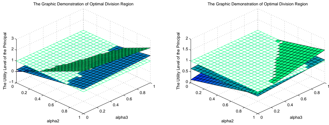
Figure 8: The principal's benefit when \gamma_1 = 0.5, \gamma_2 = 0.1, w = 0.5 (left) and \gamma_1 = 0.5, \gamma_2 = 0.9, w = 0.5 (right). The green-blue surface with black grid is the utility under agent 2 control, the white surface with green grid is under agent 1 control and the dark green one is her utility under separation.
