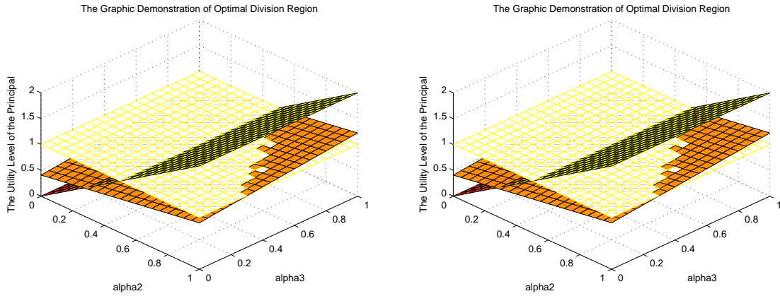
Figure 9: The principal's benefit when \gamma_1 = 0.5, \gamma_2 = 0.5, w = 0.1 (left) and \gamma_1 = 0.5, \gamma_2 = 0.5, w = 0.9 (right). The yellow-red surface with black grid is the utility under agent 2 control, the white surface with yellow grid is under agent 1 control and the orange one is her utility under separation.
