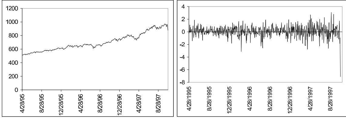
Figure 1: Data: S&P500 index and log-returns (expressed in percent).
