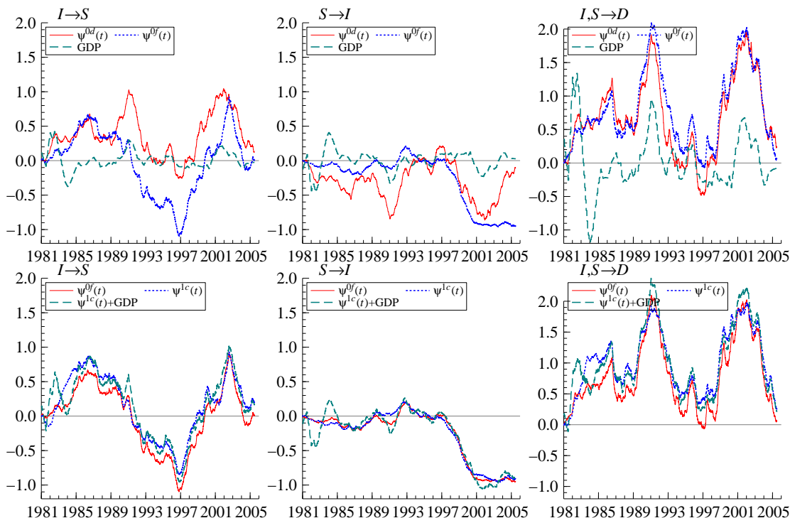
Figure 4: Estimates of the common risk factor \psi(t) (model 1c)
