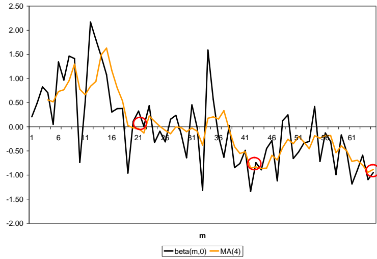
Figure 1: \beta_{m,0} for m = 1, \dots, 65
