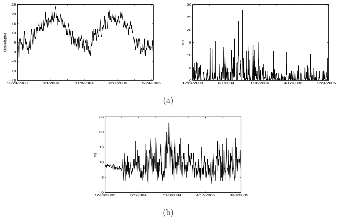
Figure 7: Weather variables: the Netherlands
