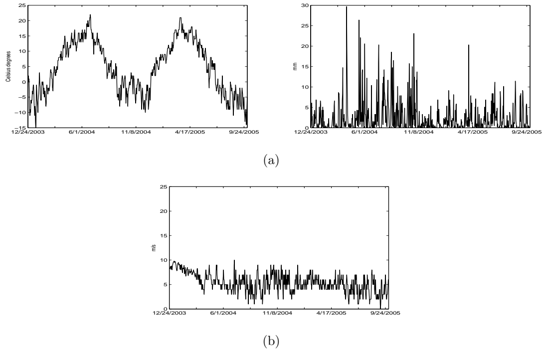
Figure 5: Weather variables: Oslo
