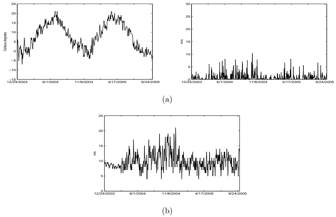
Figure 6: Weather variables: Eastern Denmark
