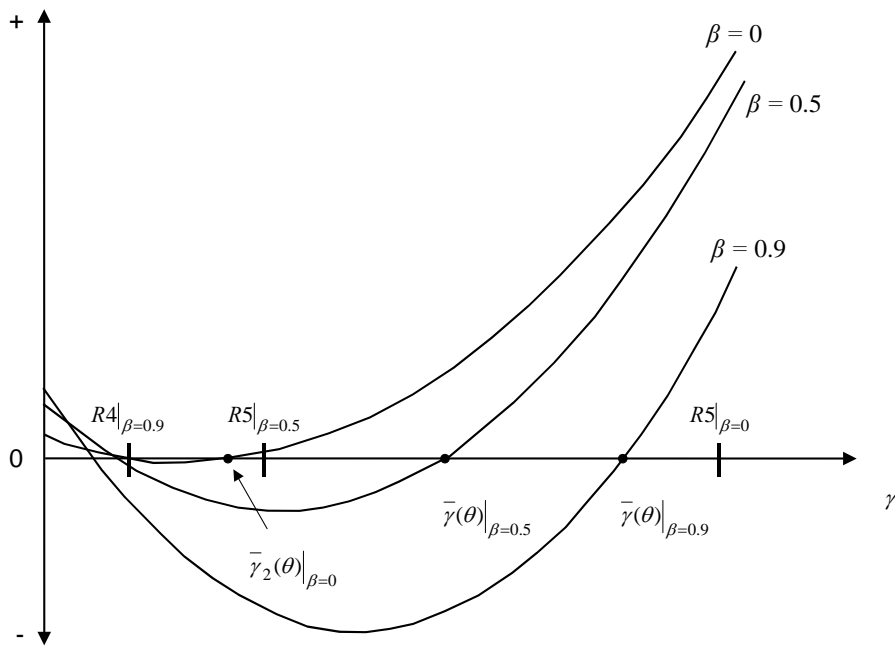
Figure 2: G(\gamma; \beta, \theta) for different levels of R&D input spillovers; a = 100 , c = 70 , \theta = 0.9 .
