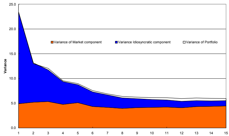
Figure 2. Variance Decomposition
