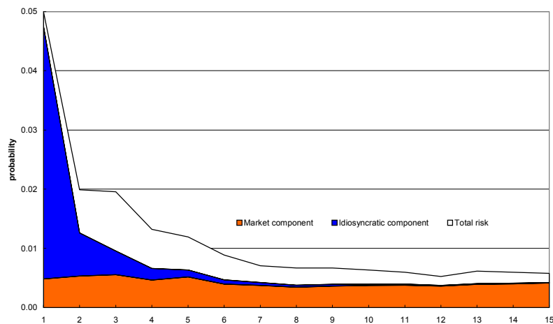
Figure 1.1 Downside Risk Decomposition at s = -7.10 (Fat-tailed case)
