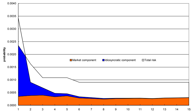
Figure 1.2 Downside Risk Decomposition at s = -15.97 (Fat-tailed case)
