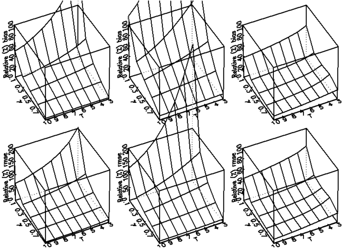
Figure 14: Inconsistent \text{GMMs}_1^{\sigma_\eta^2/\sigma_\epsilon^2} at N = 100 ; \phi = 0.5 ; \psi = 0.5, 1, 5 .
