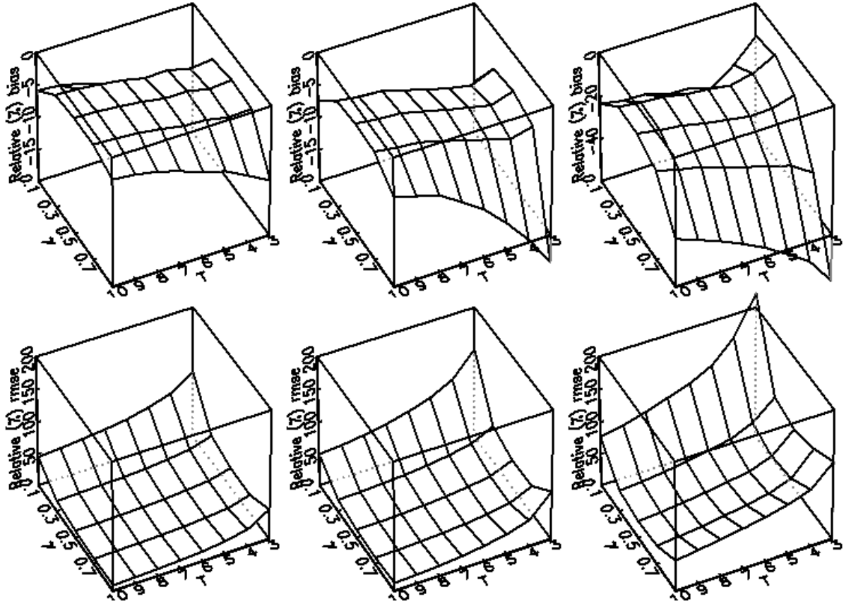
Figure 10: \text{GMM}_1^{BK} at N = 100 ; \phi = 1 ; \psi = 0, 1, 5 .
