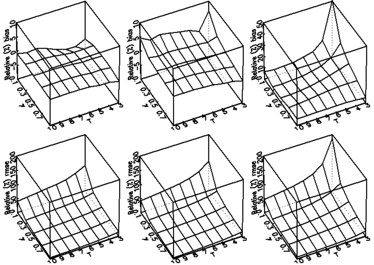
Figure 6: \text{GMMS}_2^{\sigma_\eta^2/\sigma_\varepsilon^2} at N = 100 ; \phi = 1 ; \psi = 0, 1, 5 .
