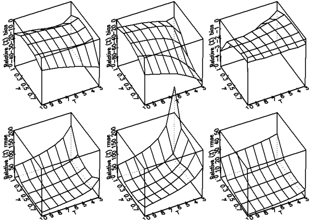
Figure 12: GMM_1^{AB} at N = 100 ; \phi = 0.5 ; \psi = 0.5, 1, 5 .
