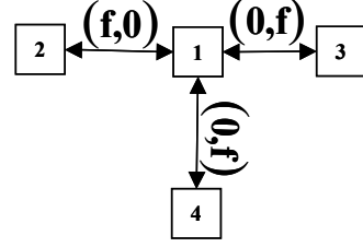
Asymmetric Efficient Outcome, 2c < f
