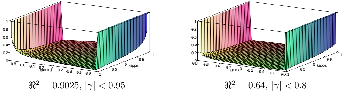
Figure 4.5: \tau_{100}^{-1}(\hat{\beta}_{\text{OLS}}) in ARX(1) model with \lambda = 0
