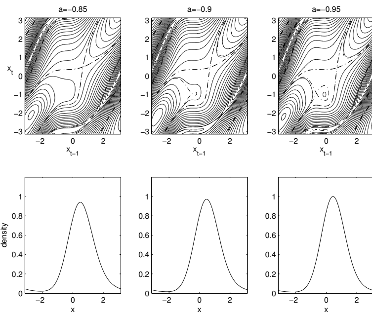
Figure 3: Level sets for the map X_t = X_{t-1} + a \sin(X_{t-1}) + 0.25 \sin^2(X_{t-1}) + 0.25 + \varepsilon_{t+1} for decreasing values of a (top panels). The dashed-dotted lines, corresponding with the critical levels of the saddle points, are added for clarity. The lower panels show the invariant probability density of X_t .
