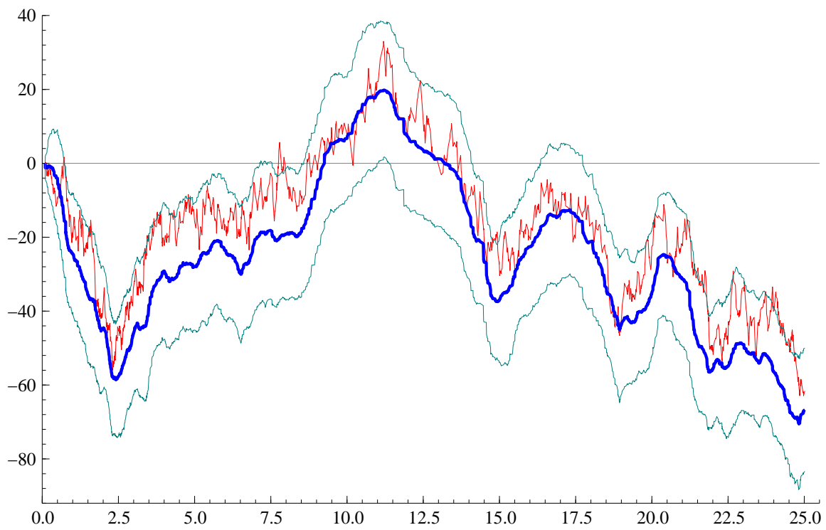
Figure 1: True versus smoothed estimate of \psi(t)
