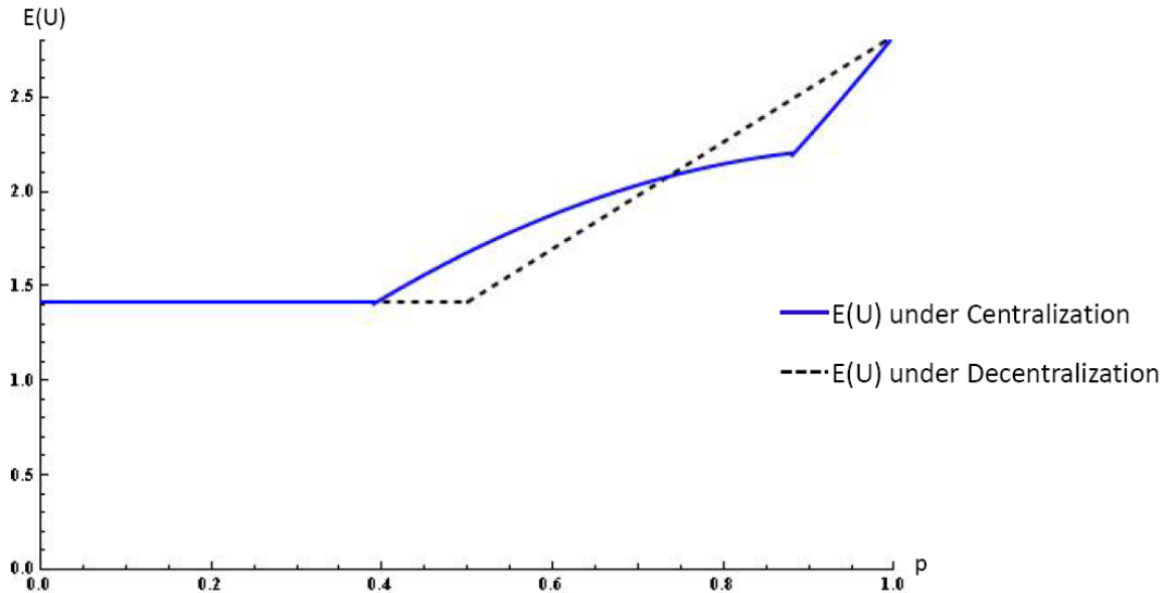
Figure 1: Expected utility under centralization and under decentralization
