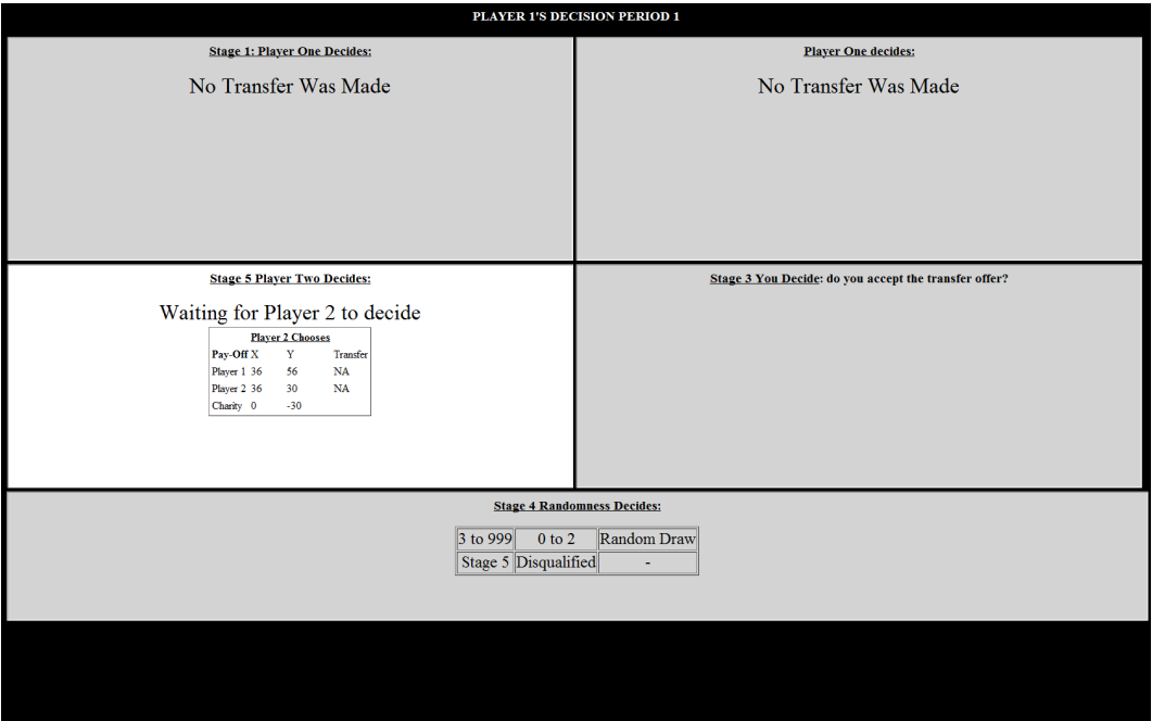
Figure 6: Decision Screen
