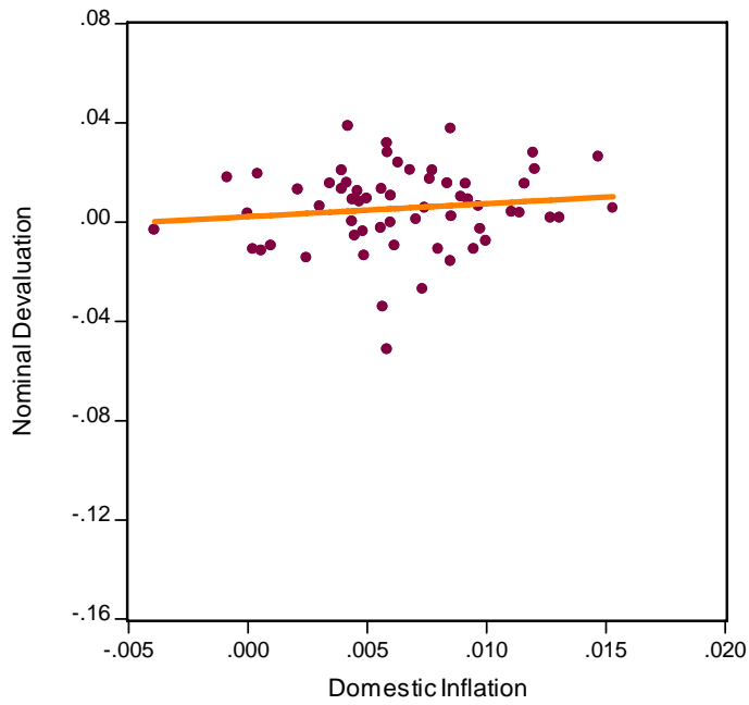
Cross-plot Domestic Inflation and Nominal Devaluation 2003-2007
