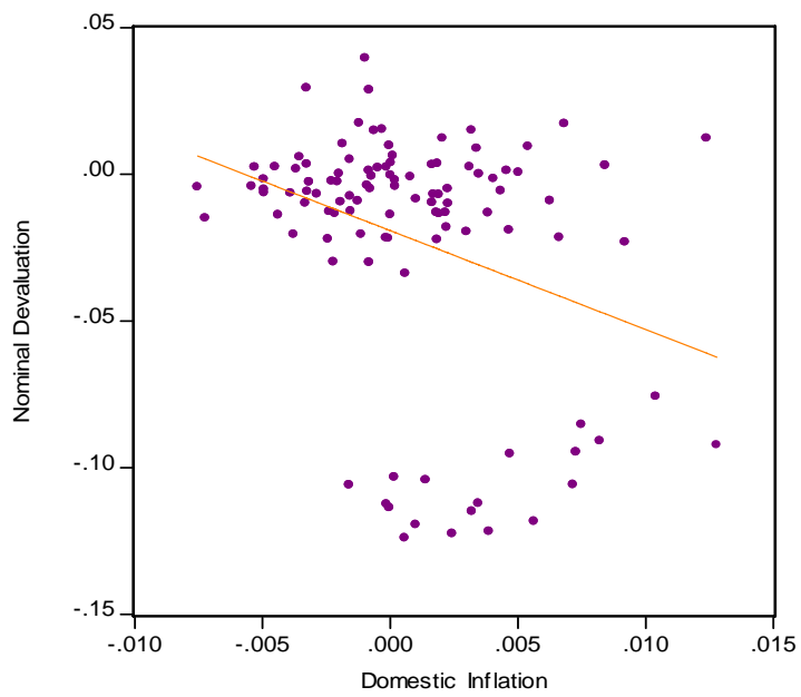
Cross-plot Domestic Inflation and Nominal Devaluation 1993-2001
