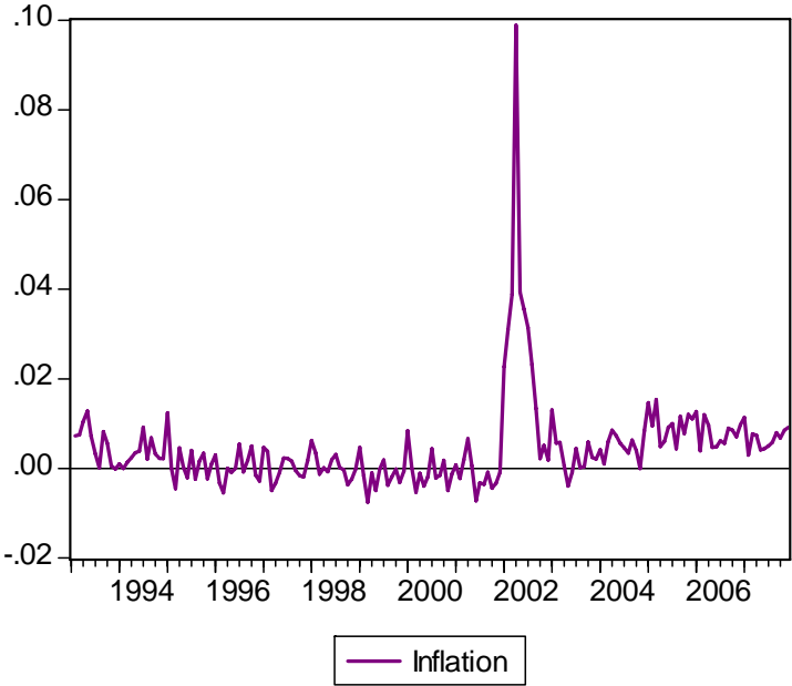
Figure 1 Time-series of Inflation 1993-2007
