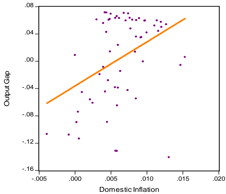
Cross-Plot Domestic Inflation and Output Gap 2003-2007
